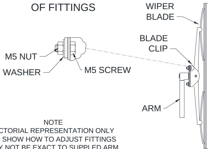
Figure - Adjusting the Wiper Blade Angle
